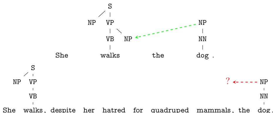
Figure 5.3: In the top example, the pipeline algorithm correctly assigned the transitive verb supertag to walks . In the bottom example, due to the long range dependency, it fails: thus, we cannot assign a head to dog .
