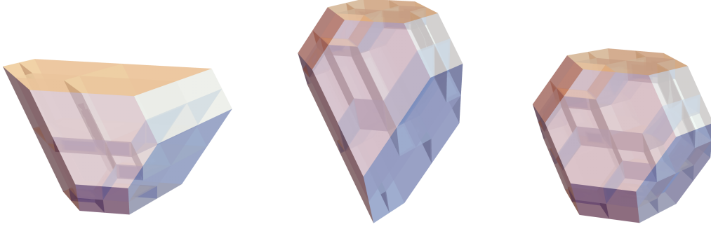
Figure 3.7: Polytopal subdivisions of some 3-dimensional operahedra, from the associahedron (left) to the permutahedron (right), given by the universal formula.
