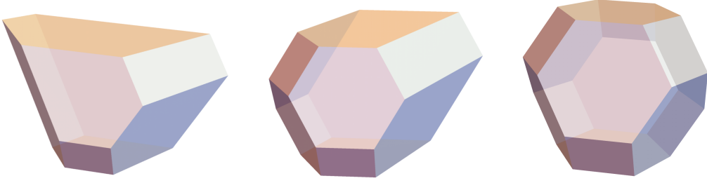
Figure 3.4: Standard weight Loday realizations of some 3-dimensional operahedra, from the associahedron (left) to the permutahedron (right).
